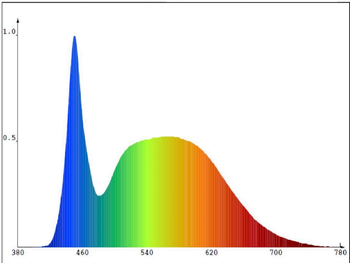
Spectral power distribution
